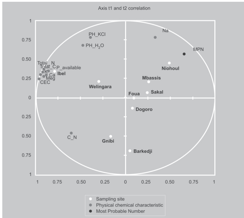
Figure 2. Tamarind parkland soil physico-chemical properties in relation to Most Probable Number (MPN), assessed from samples in three agro-ecological zones of Senegal.
