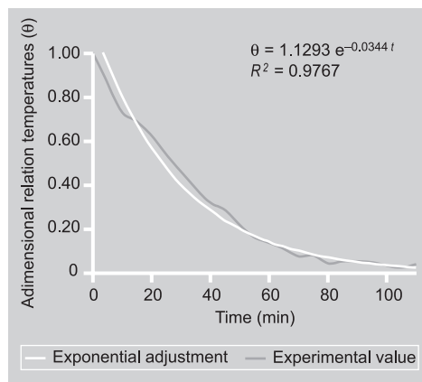
Figure 2. Distribution of experimental temperatures and curve adjustment for precooling figs packed in a carton box ( v = 2.0 \text{ m} \cdot \text{s}^{-1} ).
